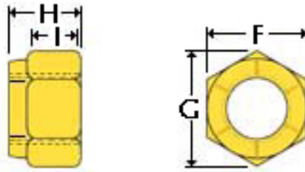
Full Height Heavy Hex
